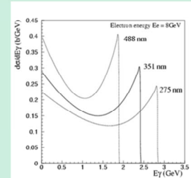
Differential cross sections for the CBS process between 8-GeV electrons and laser photons
