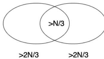
Figure 2: The intersection of two quorums must be greater than N/3 .
