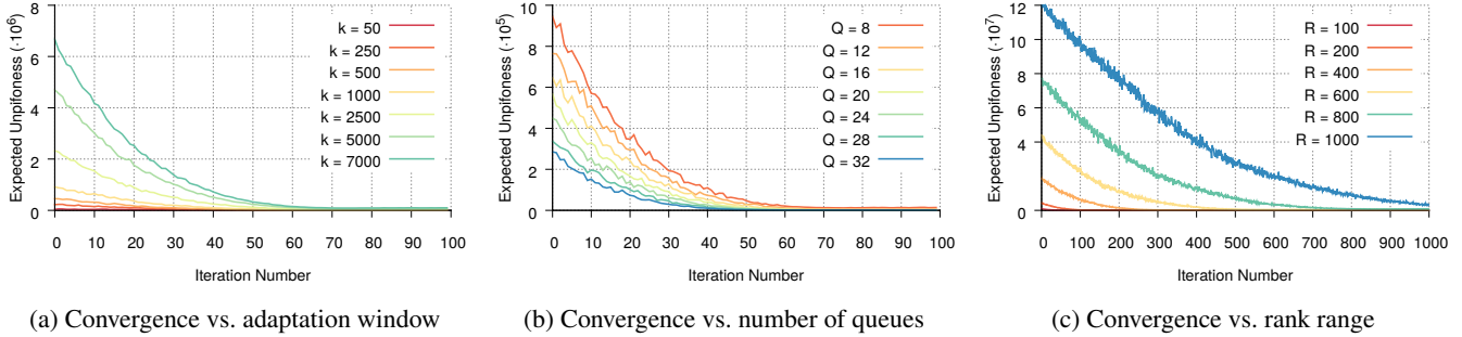
Figure 14: Greedy algorithm adaptation microbenchmark.
