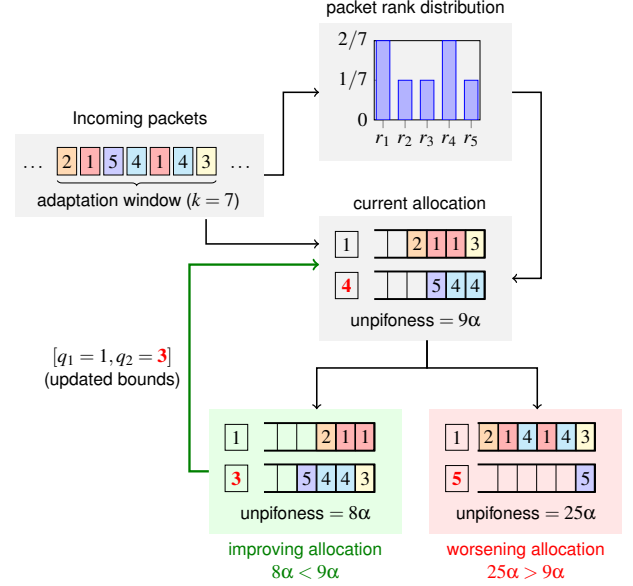
Figure 4: The gradient-based algorithm greedily minimizes the expected unpfiness .
