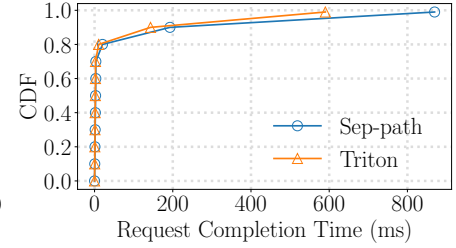
Figure 16: Nginx RCT (short conn)
