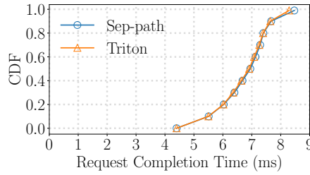
Figure 15: Nginx RCT (long conn)
