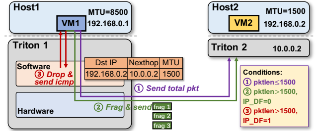
Figure 6: Triton ensures connectivity in multi-MTU scenarios. VM2 acts as a stock VM that only supports 1500 MTU.
