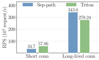
Figure 14: Nginx RPS Performance
