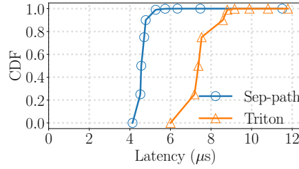
Figure 9: Latency overhead
