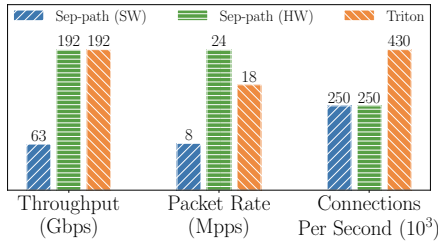
Figure 8: Overall performance
