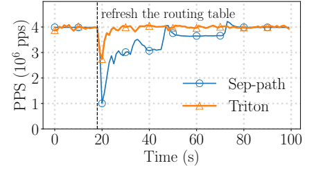
Figure 10: Predictable performance
