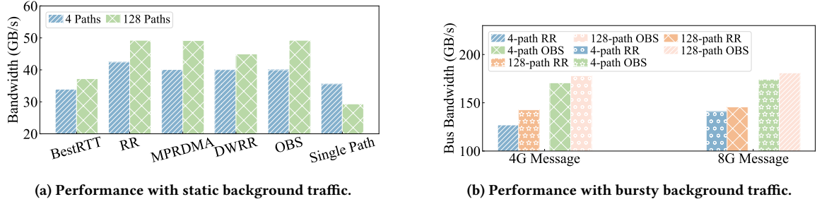
Figure 10: AllReduce performance under different background traffic conditions: static and bursty.
