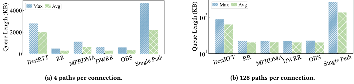
Figure 9: Queue depth for permutation traffic, comparing performance with 4 paths versus 128 paths per connection.
