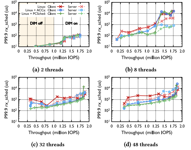
Figure 10: rx\_sched still dominates the end-to-end P99.9 latency with increasing in-flight requests. When there are two threads per core (one per logical core), rx\_sched increases only mildly with increasing in-flight requests, primarily due to additional queuing in the TCP receive buffer rather than scheduling contention. More discussion in §3.3.
