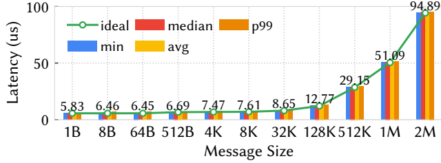
Figure 19: Message Size Scaling
