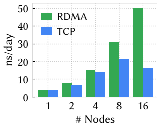
Figure 27: Gromacs
