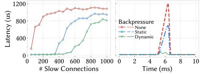
Figure 24: Isolation via fine-grained backpressure
