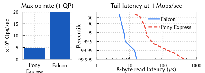
Figure 1: Comparing the limits of SW-based stacks
