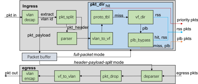
Figure A.1: Basic Pipeline
