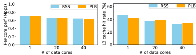
Figure 4: Perf comparison of VPC-Internet service.
