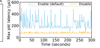
Figure 17: Impact of NUMA balancing.
