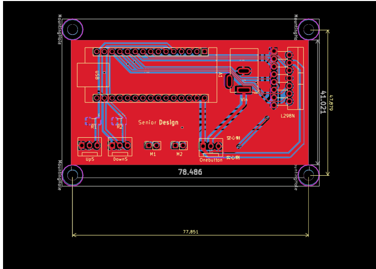
Figure 9: PCB Layout
