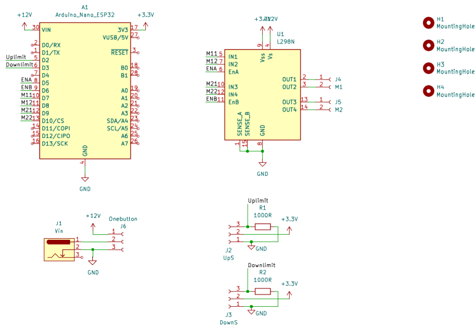
Figure 10: PCB Schematic
