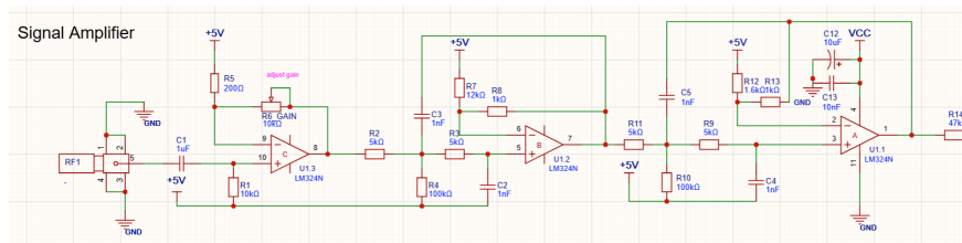
Figure 10: Signal amplifier
