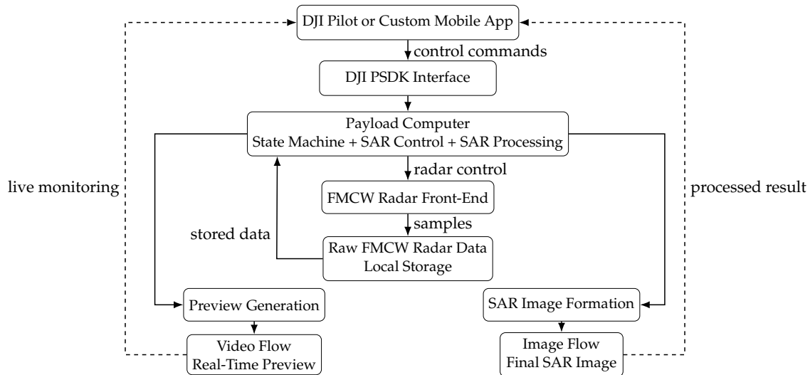
Figure 5: Control path, real-time preview flow, and SAR image flow
