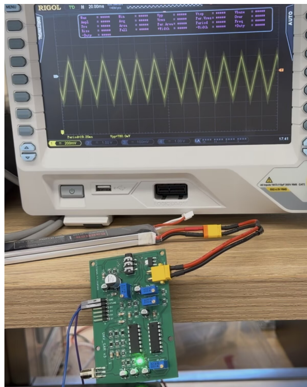
Figure 12: Wave generation testing
