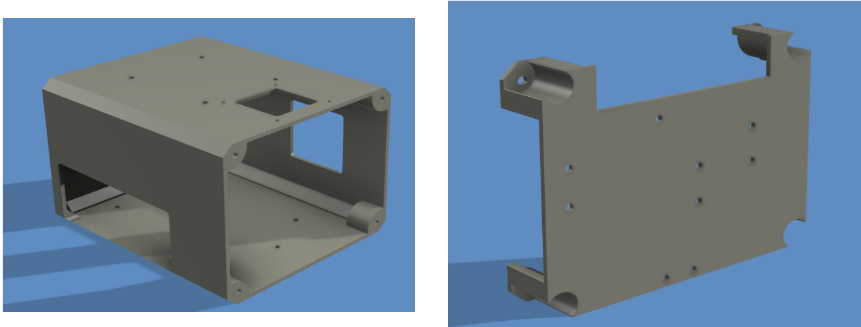
Figure 7: 3D CAD renderings of the enclosure body and detachable cover
