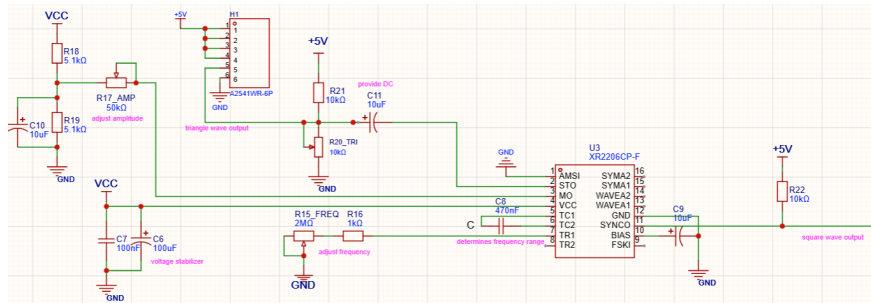
Figure 9: Wave generator
