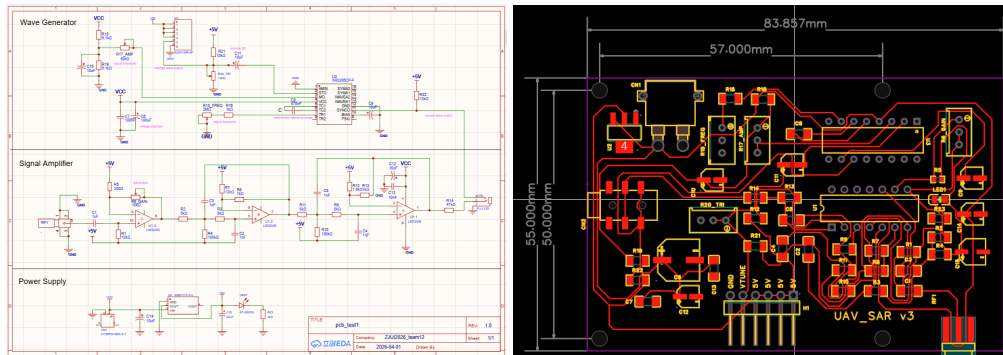
Figure 8: Our PCB
