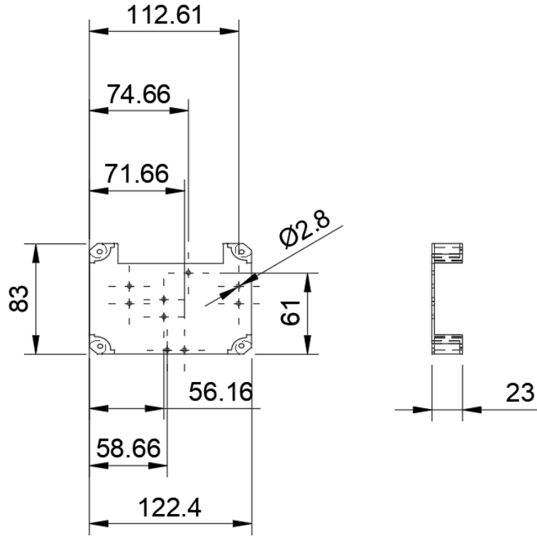
Figure 16: Dimensional layout of the detachable enclosure cover
