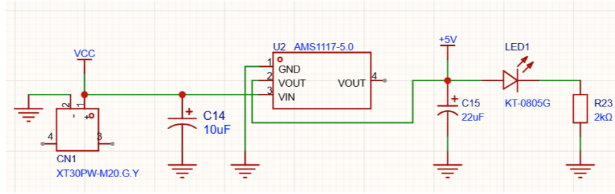
Figure 11: Power supply
