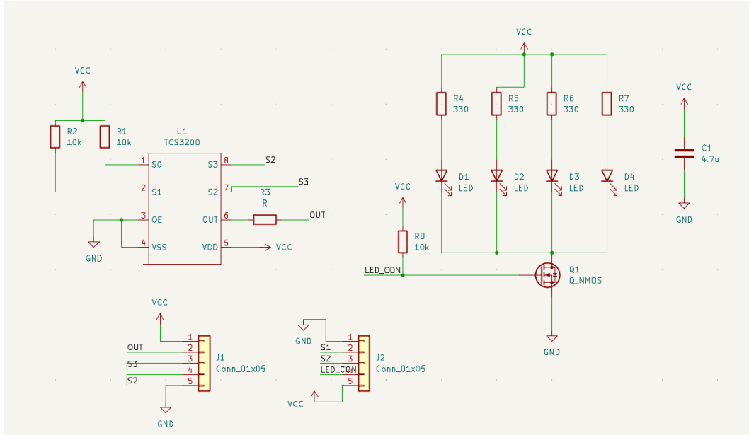
Figure 3: Auxiliary object-presence sensing circuit.
