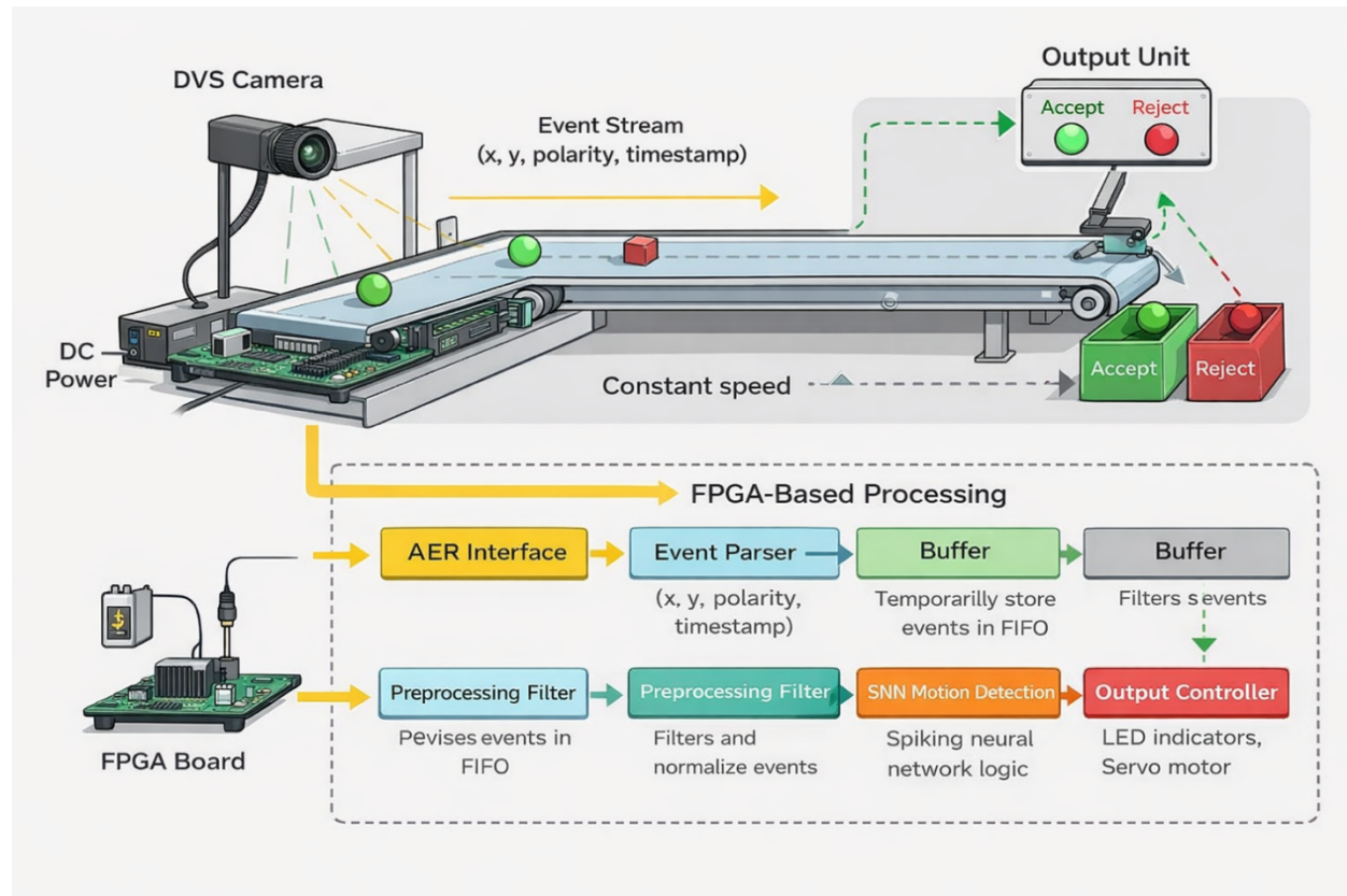
Figure 1. Visual overview of the proposed smart package inspection and sorting system. Packaged items move on a conveyor under a DVS camera. The event stream is processed by the FPGA in real time, and the classification result drives an LED indicator and a sorting actuator to separate acceptable packages from damaged packages.
