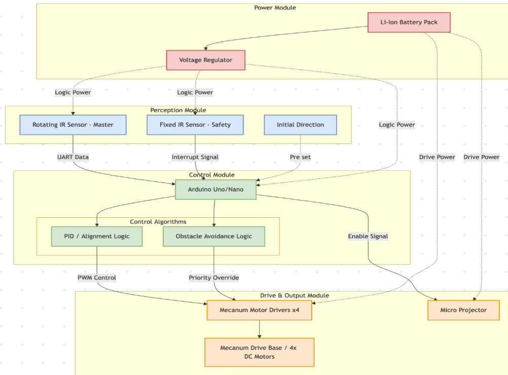
Figure: The block diagram of the whole system
