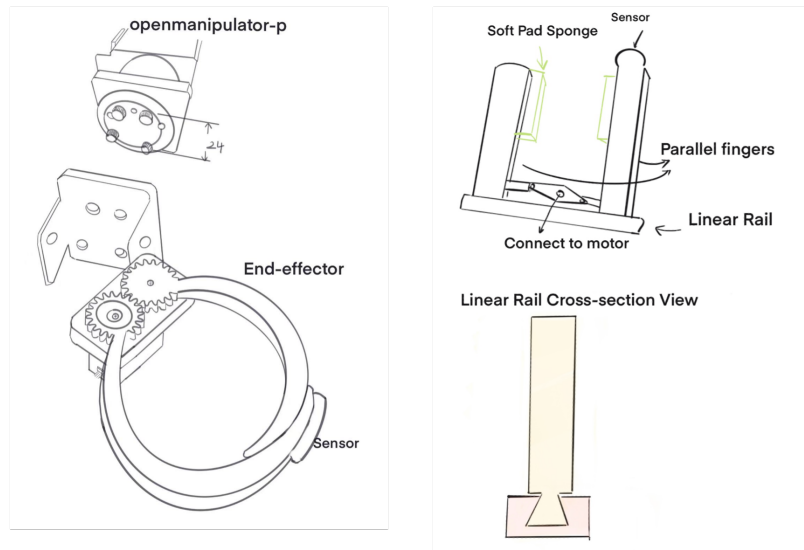
Figure 3: Curved Gripper (left) v.s. Parallel Gripper (right)
