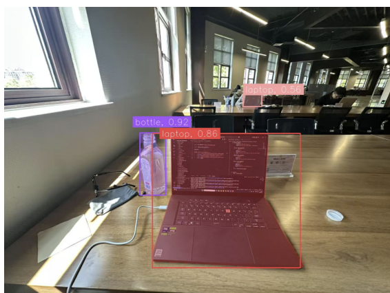
(c) YOLOE-11L
