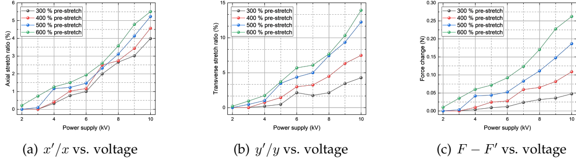
Figure 11: Results of the pre-stretching experiment for linear DE-HASEL actuators.
