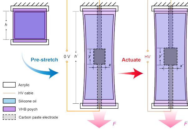
Figure 9: Illustration of the pre-stretching experiment for the DE-HASEL actuator.
