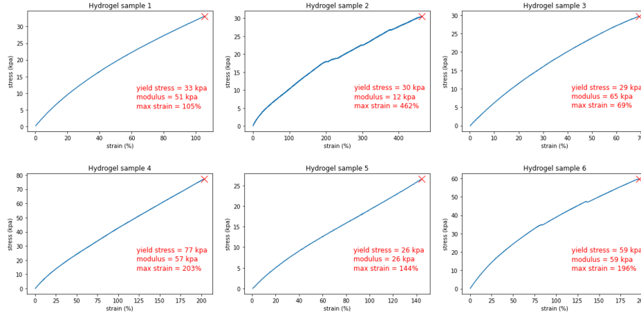
Figure 13: Illustration of the strain-stress digrams for the hydrogel electrode layer.
