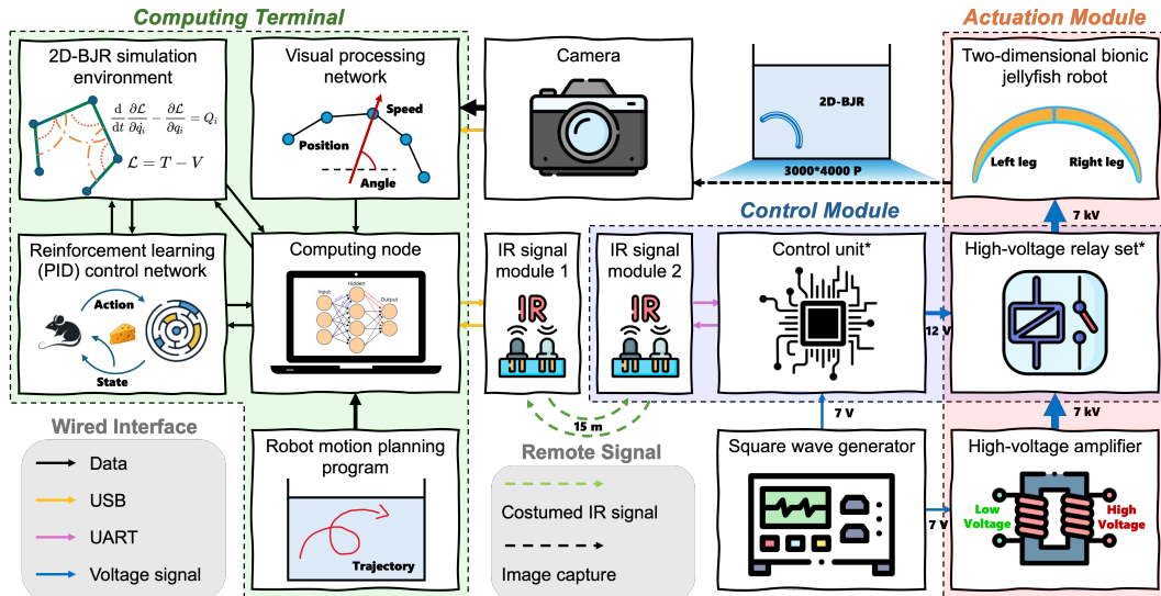
Figure 1: Block Diagram of 2D-BJR system
