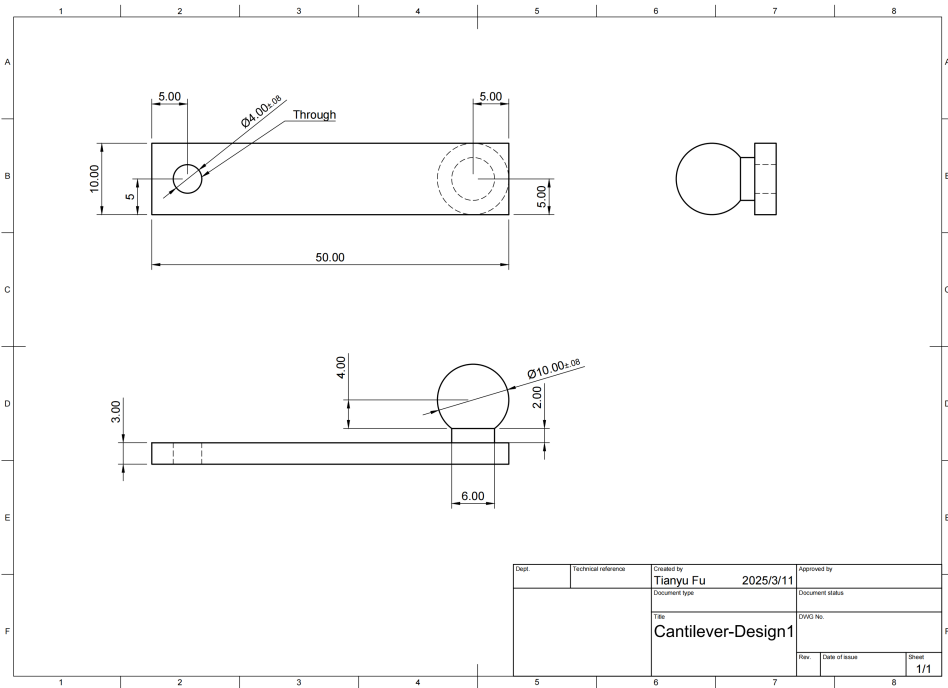
Figure 12: Orthographic Views of the Cantilever
