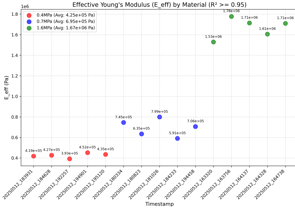
Figure 8: Scatter dot diagram comparing the measured elastic moduli of PDMS samples with known reference values.
