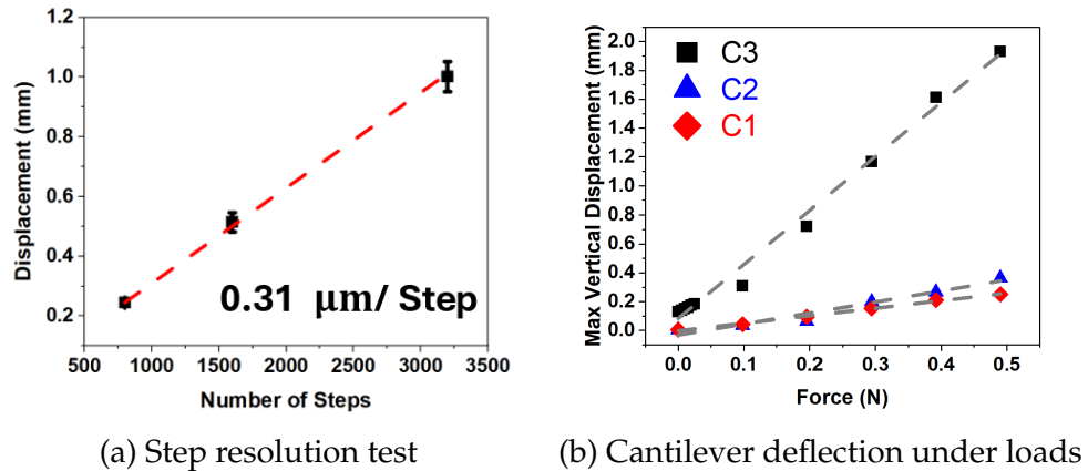
Figure 10: Mechanical module verification results
