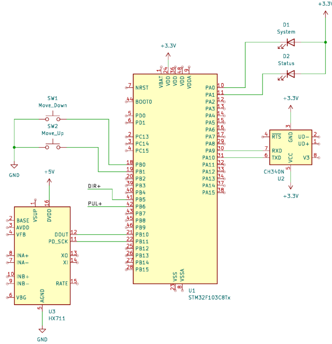
Figure 5: Schematic for STM32 Control System
