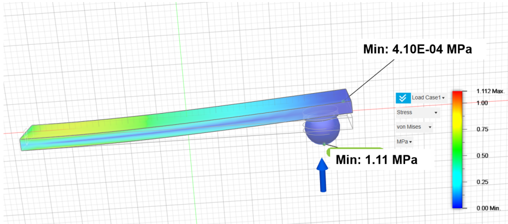
Figure 15: Stress Simulation
