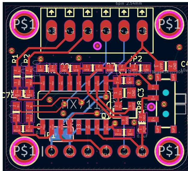
Figure 16: PCB layout
