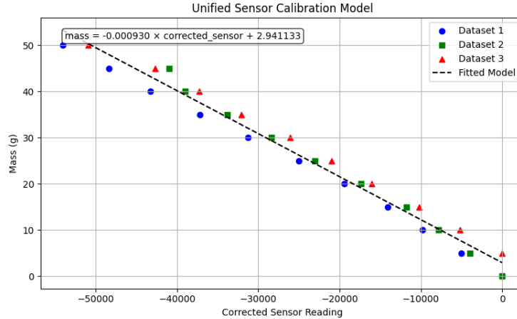
Figure 6: Calibration Curve: The linear relationship between corrected sensor readings and applied mass, based on the derived model.
