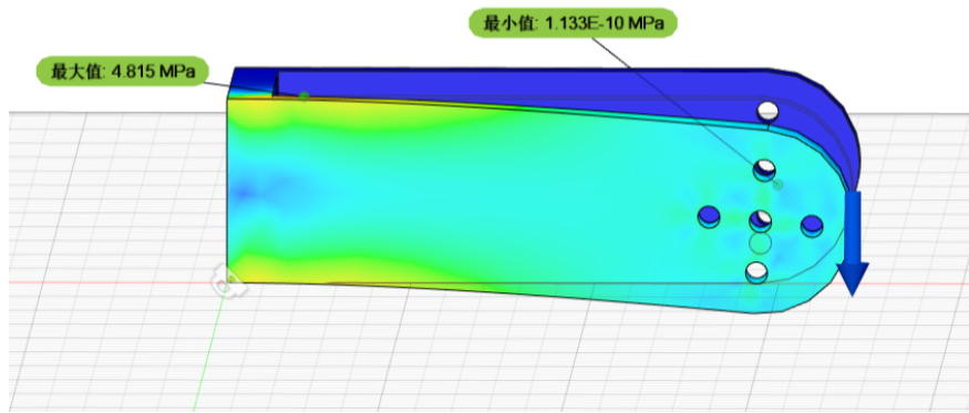
Figure 13: FEA result of the segment
