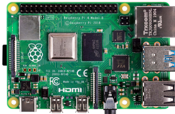
Figure 11: Raspberry Pi 4 Model B
