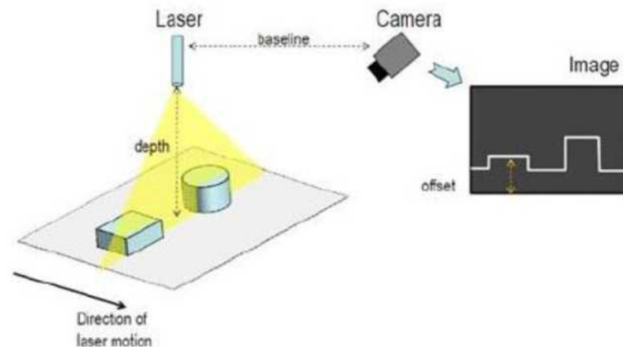
Figure 9: 3D Camera
