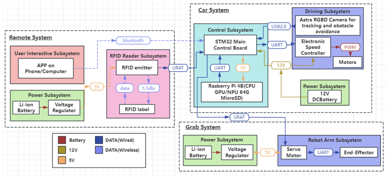
Figure 5: Block Diagram
