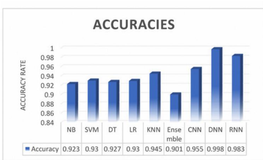
Figure 3: Accuracies
