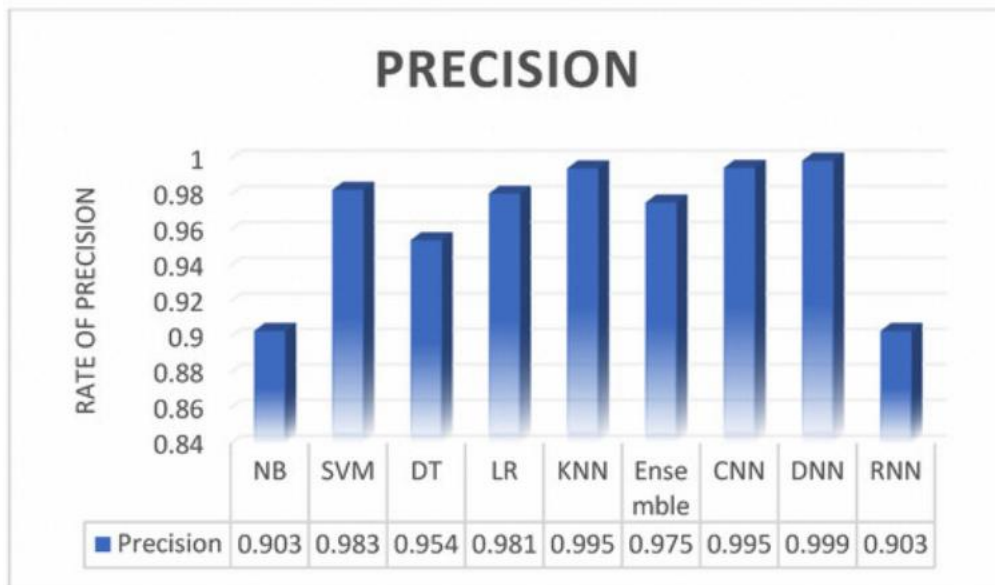
Figure 4: Precision
