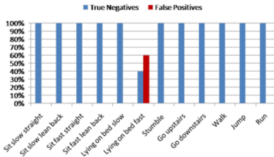
Figure 5: Accuracies for Wearable Device Detector
