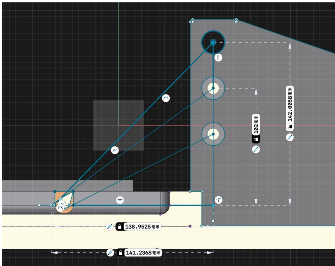
Figure10. Film deposition Angle and horizontal distance of tank
