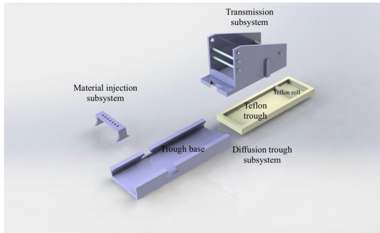
Figure2. Detailed sketch of unassembled design
