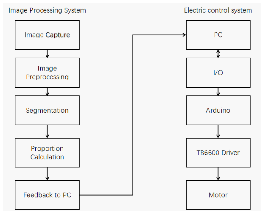
Figure9. Block diagram between electric control and image processing subsystem
