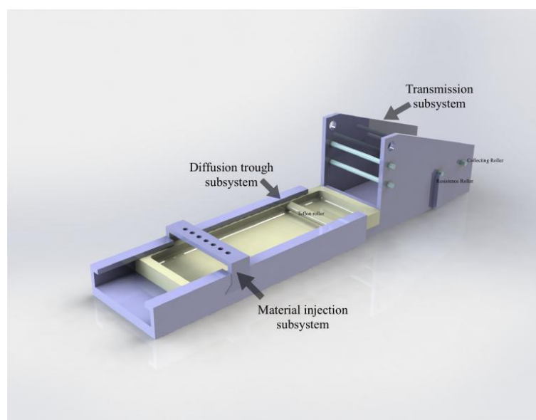
Figure1. Detailed design sketches for assembly completion
