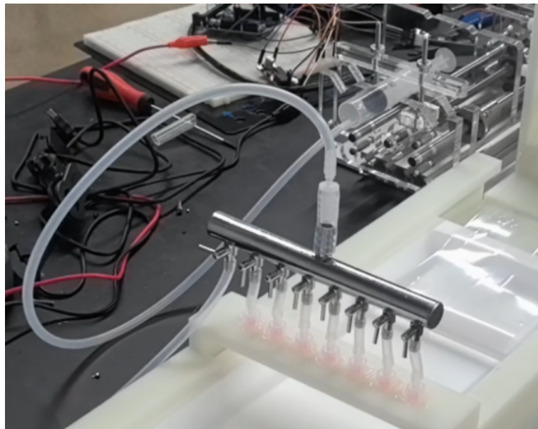
Figure7.Preliminary design of material addition subsystem
