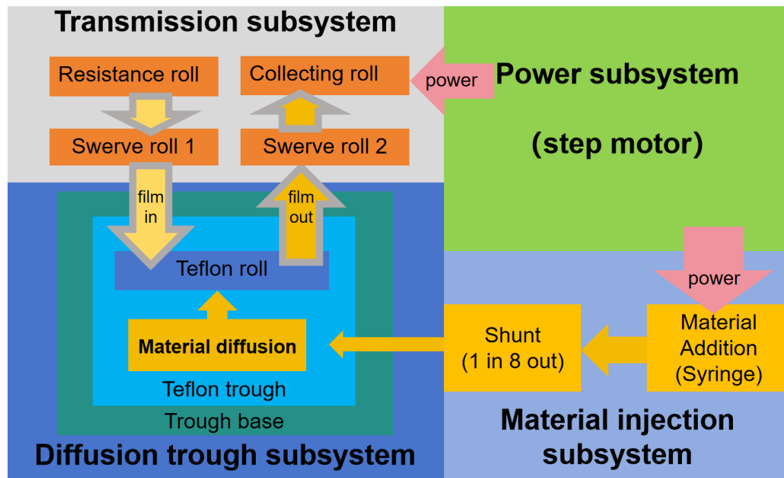
Figure 3. Block diagram between electric control and deposition tank subsystem
