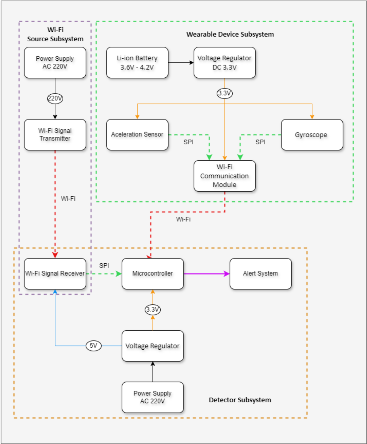
Figure 2: Block Diagram
