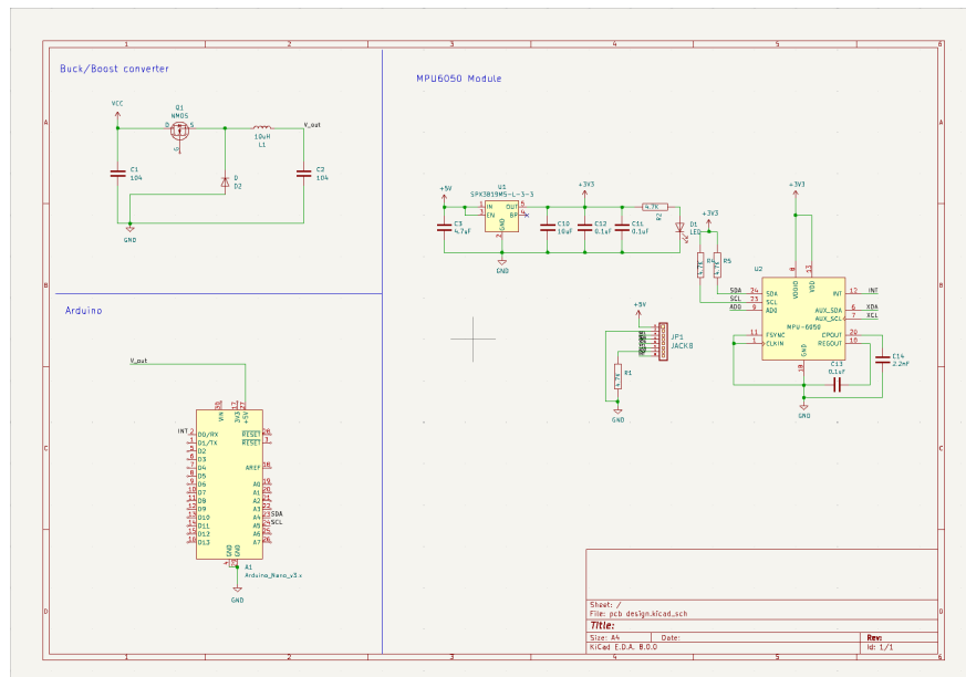
Figure 4: PCB Design
