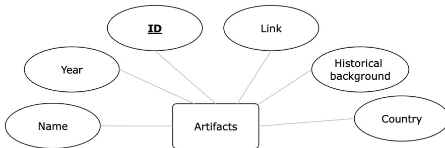
Figure 5: Entity-Relationship Diagram
