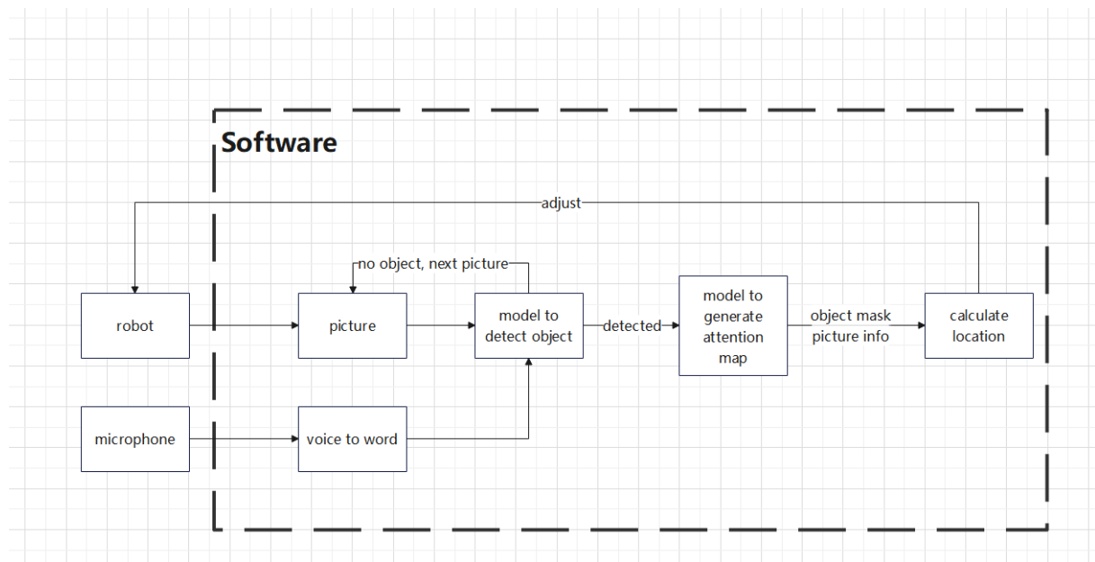
Figure 2: Block Diagram for the Software Component
