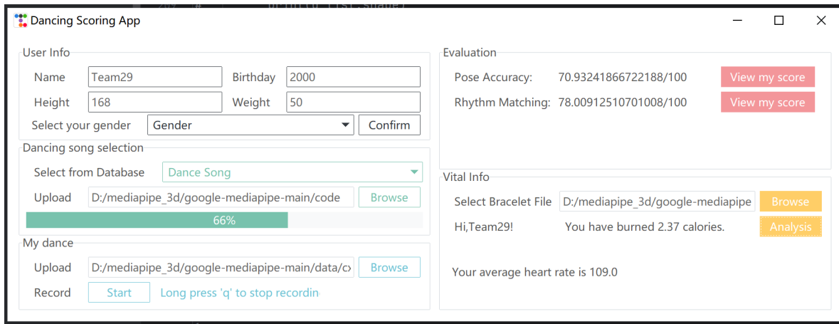
Figure 16: GUI Interface
