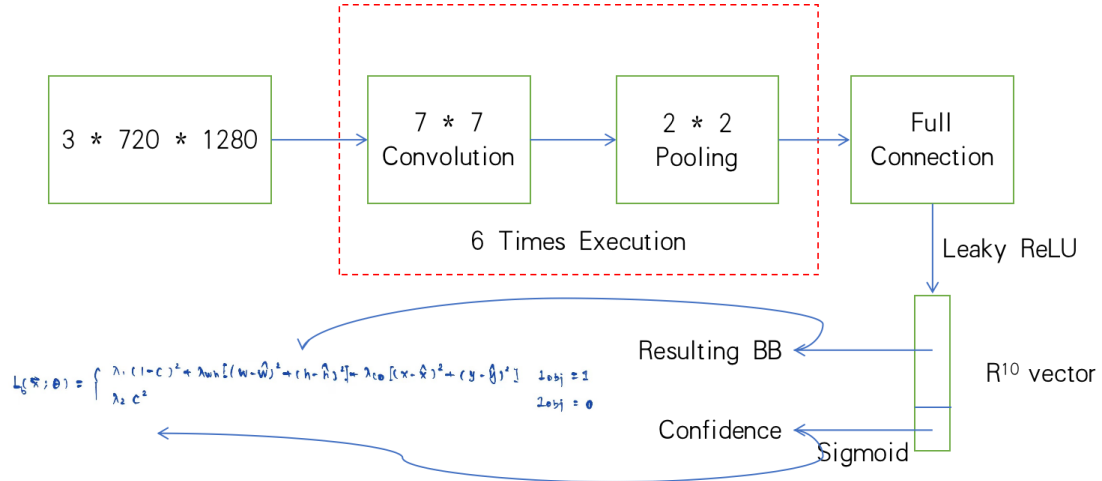
Figure 4: Network Design
