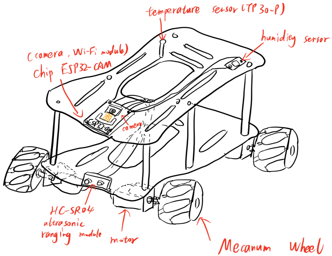
Figure 3: Physical Design
