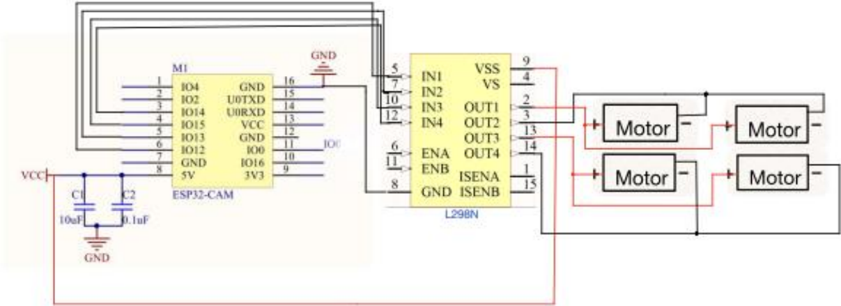
Figure 9: Control system schematic
