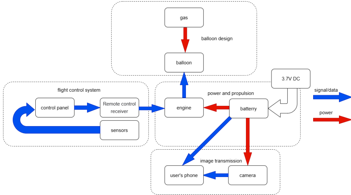
Figure 2: Block diagram
