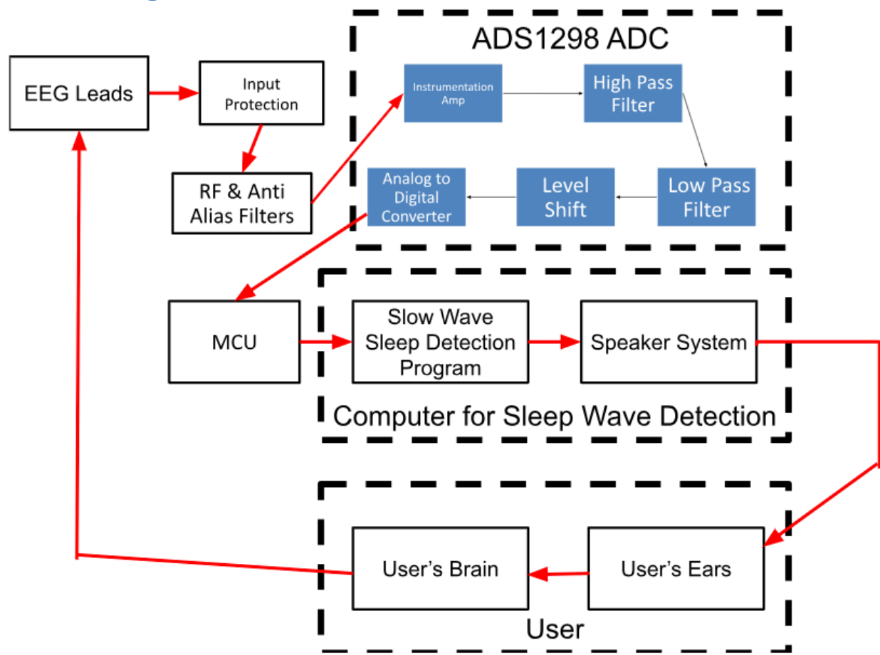
Figure 2: Block Diagram
