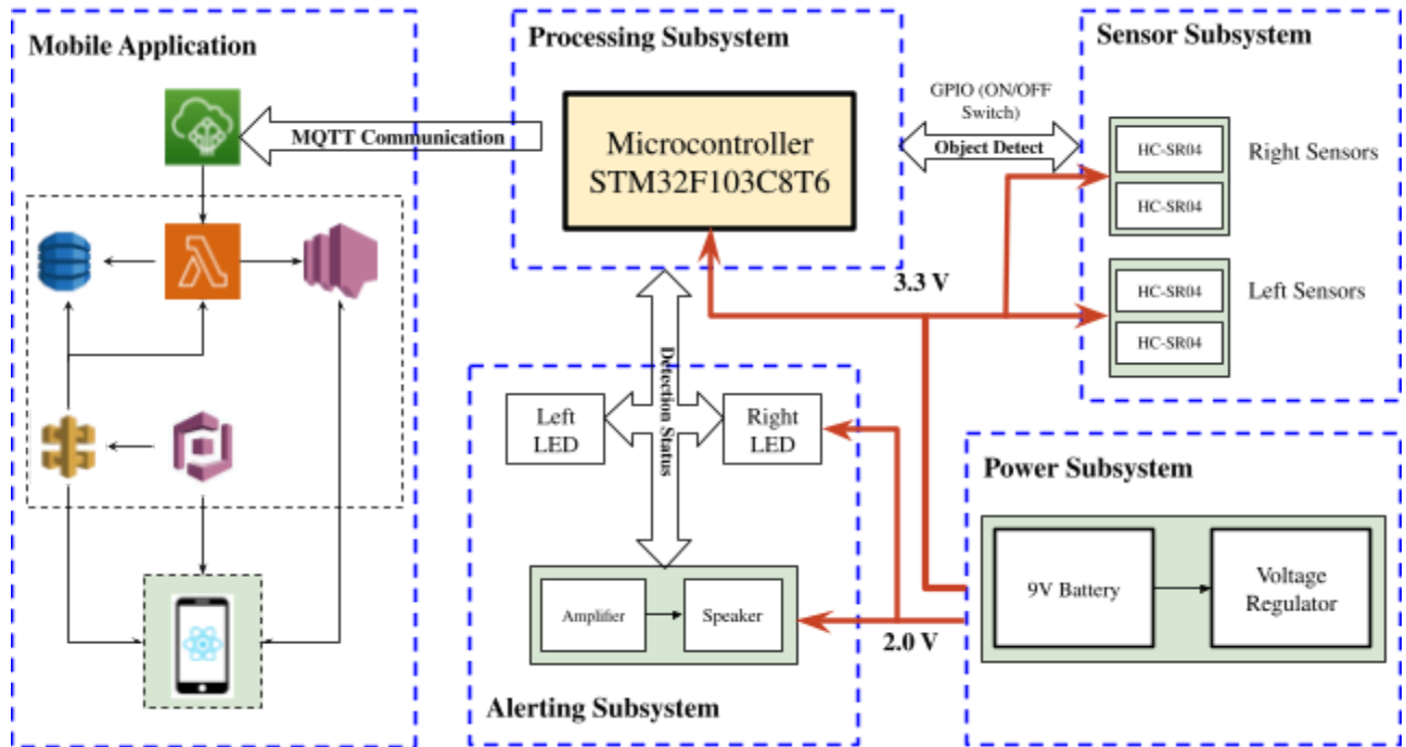
Figure 4: Block Diagram
