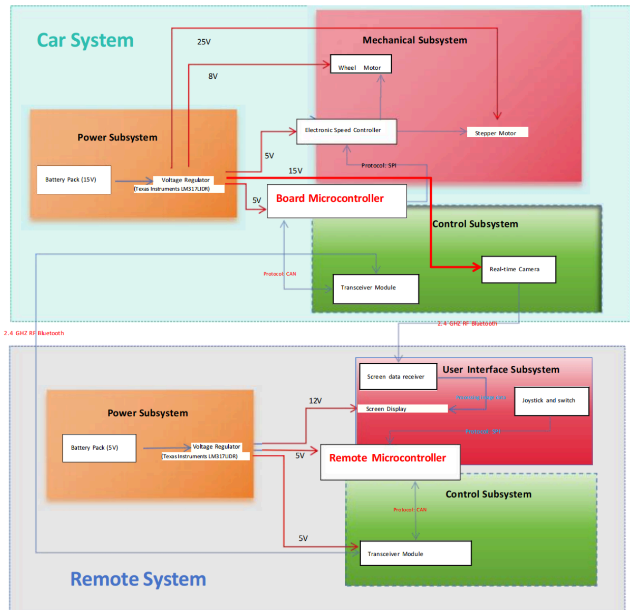
Block diagram
