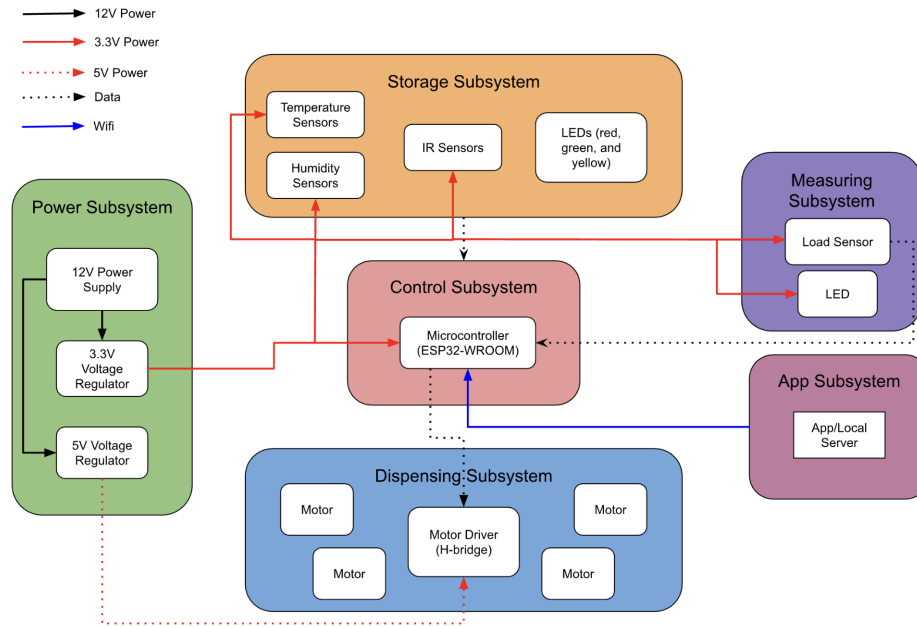
Figure 2: Proposed block diagram
