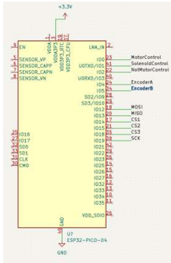
Figure 5: Microcontroller of Control Subsystem
