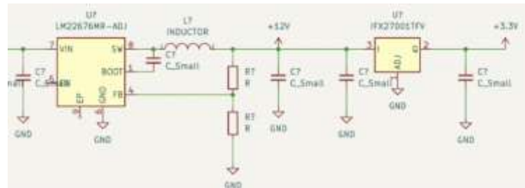
Figure 4: Circuitry of Power Subsystem
