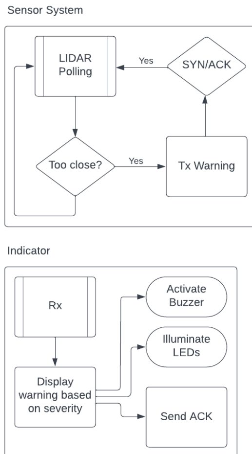
Figure 2.1-2: Flowchart for Sensor and Indicator Systems
