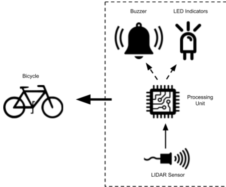
Figure 1.2-1: Hazard detection integrated on bicycle.
