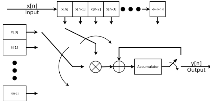
Figure 8: Low area FIR filter [8]
