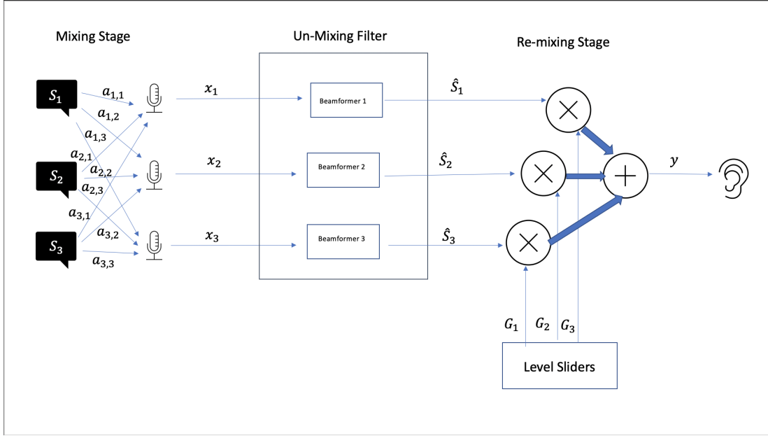
Figure 9: Forward Model of signals propagating through the Augmented Listening Platform
