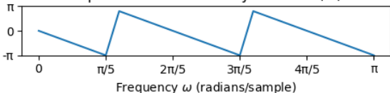
Phase Response of a Pure-Delay Filter \angle G(\omega) = -5\omega
