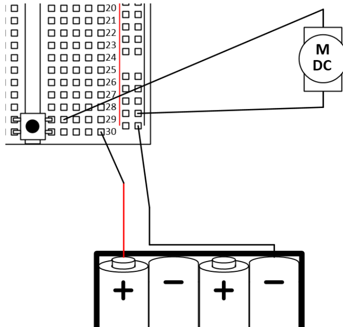
Figure 8: Circuit schematic for button-controlled motors.
