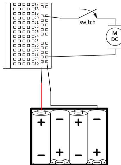
Figure 7: Example physical diagram for switching motors using the snap-action switch. The second wire on the switch should be the “normally-open” (no) connector.
