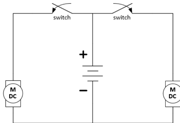
Figure 6: Circuit schematic for switching motors.
