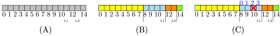
Figure 43.2: (A) m = 15 . (B) The block decomposition. (C) If X = 10 , then the extraction output is 2 in base 2, using 2 bits – that is 10.
