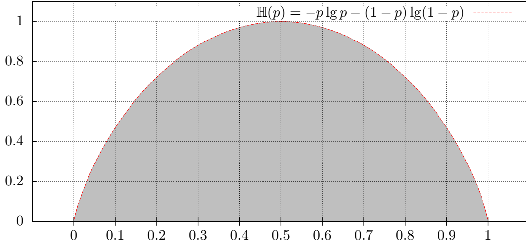
Figure 43.1: The binary entropy function.
