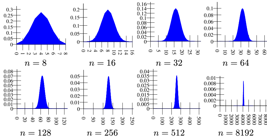
Figure 15.1: The binomial distribution for different values of n . It pretty quickly concentrates around its expectation.
