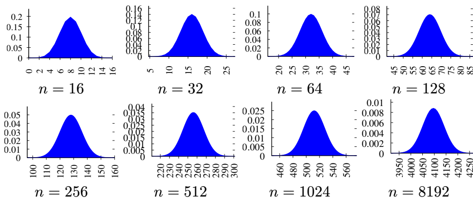
Figure 15.2: The “middle” of the binomial distribution for different values of n . It very quickly converges to the normal distribution (under appropriate rescaling and translation).
