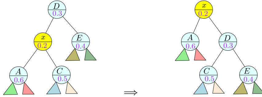
Figure 14.1: RotateRight : Rotate right in action. Importantly, after the rotation the priorities are ordered correctly (at least locally for this subtree).
