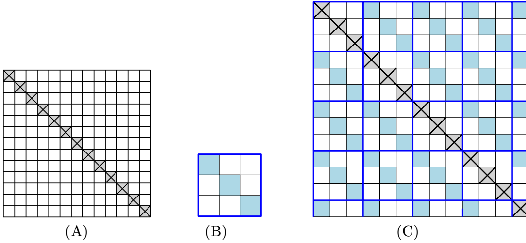
Figure 10.2: Explanation of the hashing scheme via figures.
