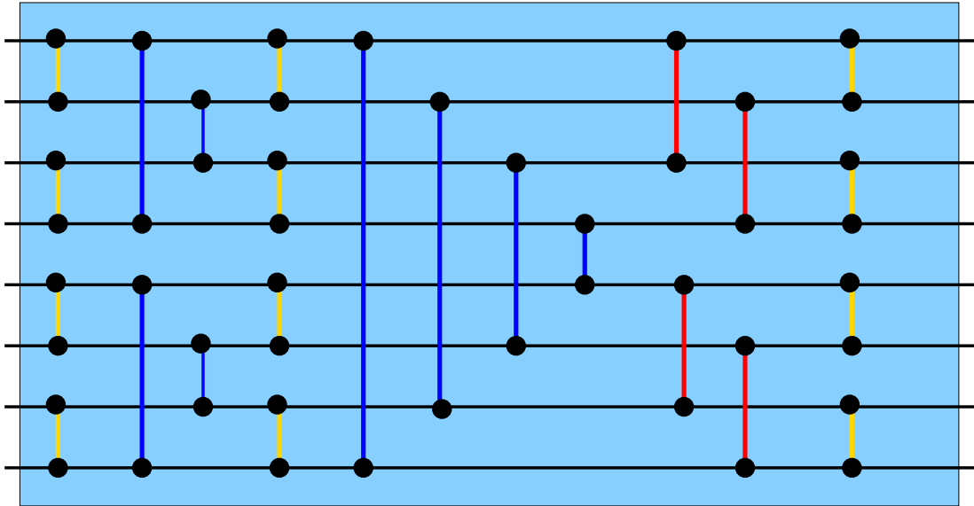
Figure 20.1: Sorter [8].
