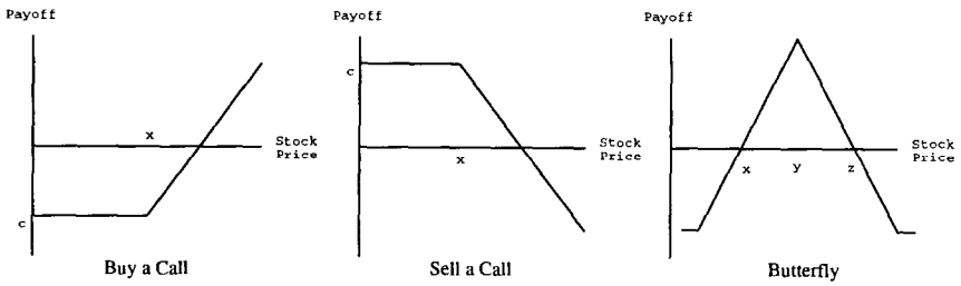
FIGURE 5. Payoff diagrams.
