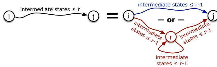
Figure 9.3. Recursive structure of the regular language L(i, j, r) .
