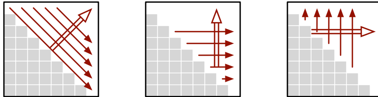
Figure 3.5. Three different evaluation orders for the optimal binary search tree problem.
