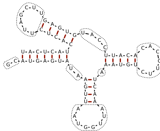
Example RNA secondary structure with 21 bonded base pairs, indicated by heavy red lines. Gaps are indicated by dotted curves. This structure has score 2^2 + 2^2 + 8^2 + 1^2 + 7^2 + 4^2 + 7^2 = 187 .
