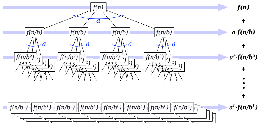
A recursion tree for the recurrence T(n) = aT(n/b) + f(n)
