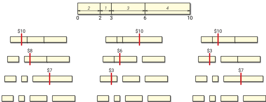
Figure 2.7. Three ways to cut a marked plank into four pieces, with total costs $25, $19, and $20.
