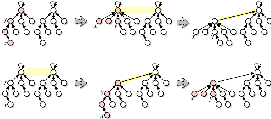
Top row: A \text{COMPRESS} followed by a \text{UNION} . Bottom row: The same operations in the opposite order.
