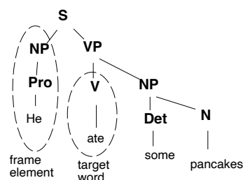
Figure 4: In this example, the path from the frame element “He” to the target word “ate” can be represented as NP \uparrow S \downarrow VP \downarrow V, with \uparrow indicating upward movement in the parse tree and \downarrow downward movement.
