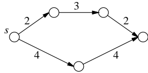
Figure 9.1. Increasing all the edge weights by 2 changes the shortest path s to t .
