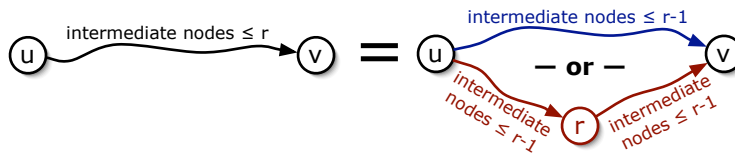
Figure 9.2. Recursive structure of the restricted shortest path \pi(u, v, r) .
