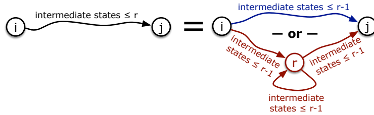
Figure 9.3. Recursive structure of the regular language L(i, j, r) .
