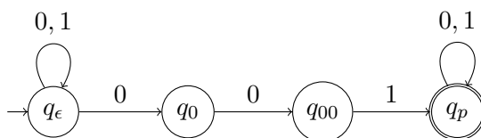
Figure 5: q_\epsilon has two 0-transitions
