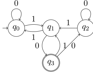
Figure 16: DFA M
