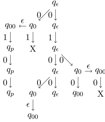
Figure 11: Computation on 0100
