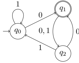
Figure 1: DFA M for question 5
