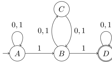
Figure 2: NFA N for question 6
